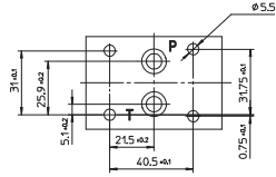
valve's surface
