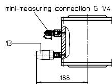
partial section A-A
